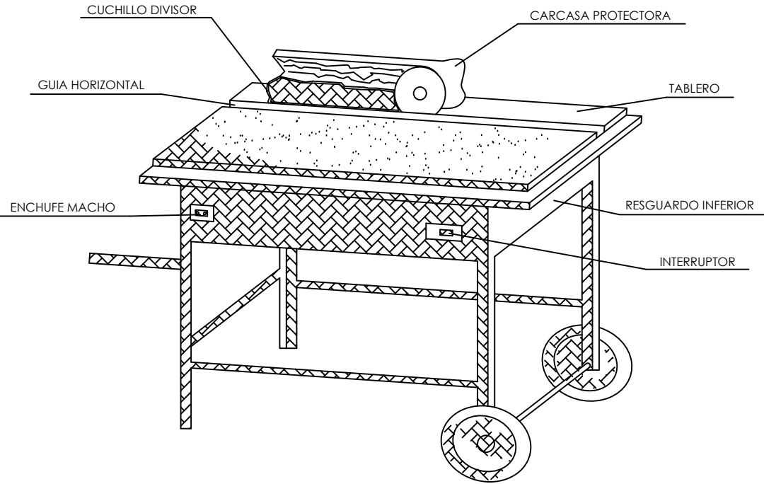
SIERRA CIRCULAR
